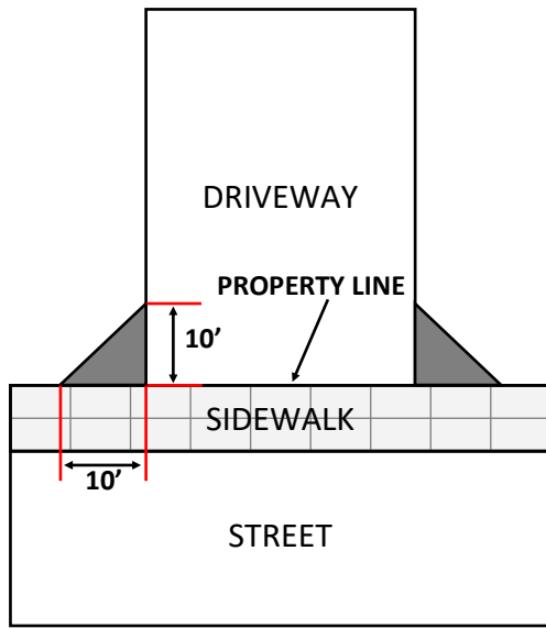
Sidewalk Example
