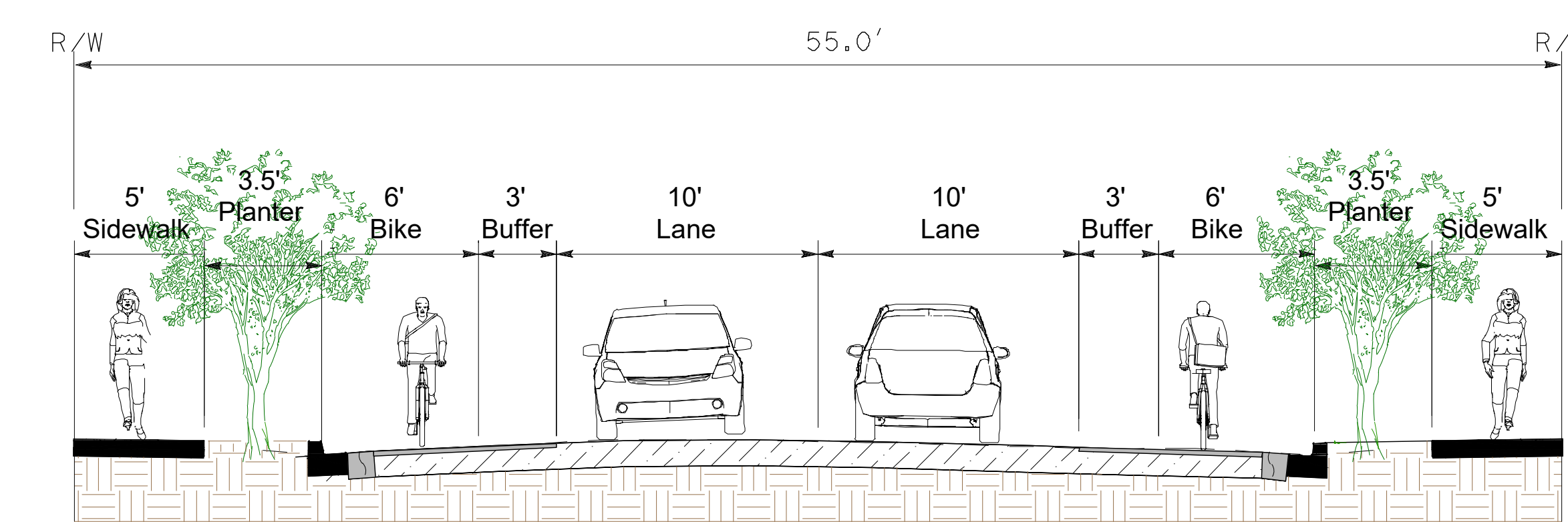
WEST OF MAGNESON LOOP SCALE: 1" = 10'
